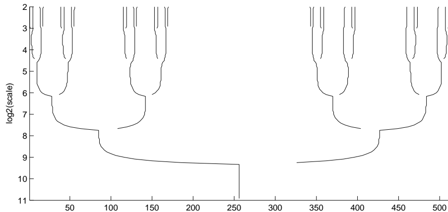
Figure 10: Devil's Staircase and its wavelet transform
